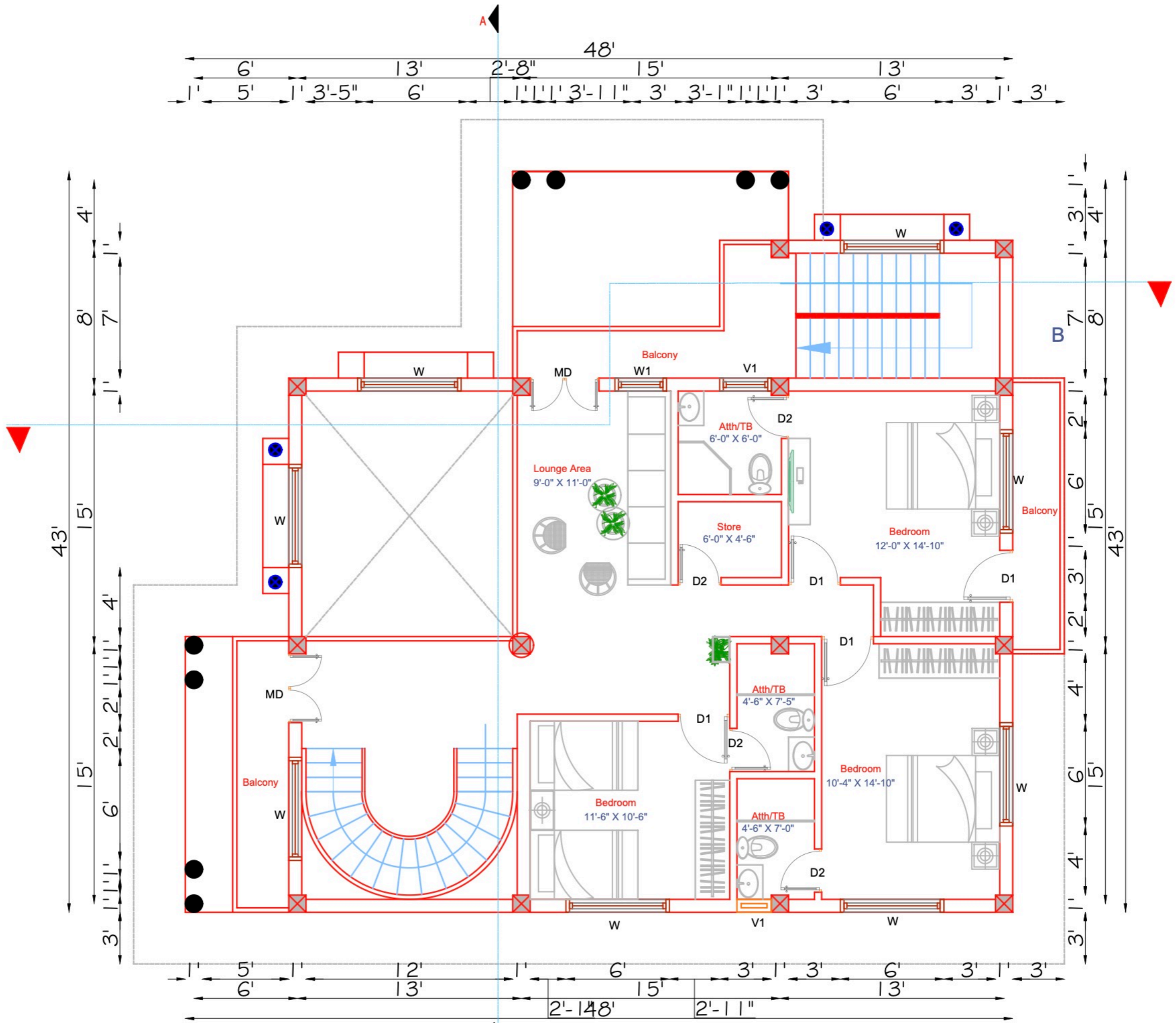
A FIRST FLOOR PLAN Built-up Area: 1694.00 Sq.Ft
