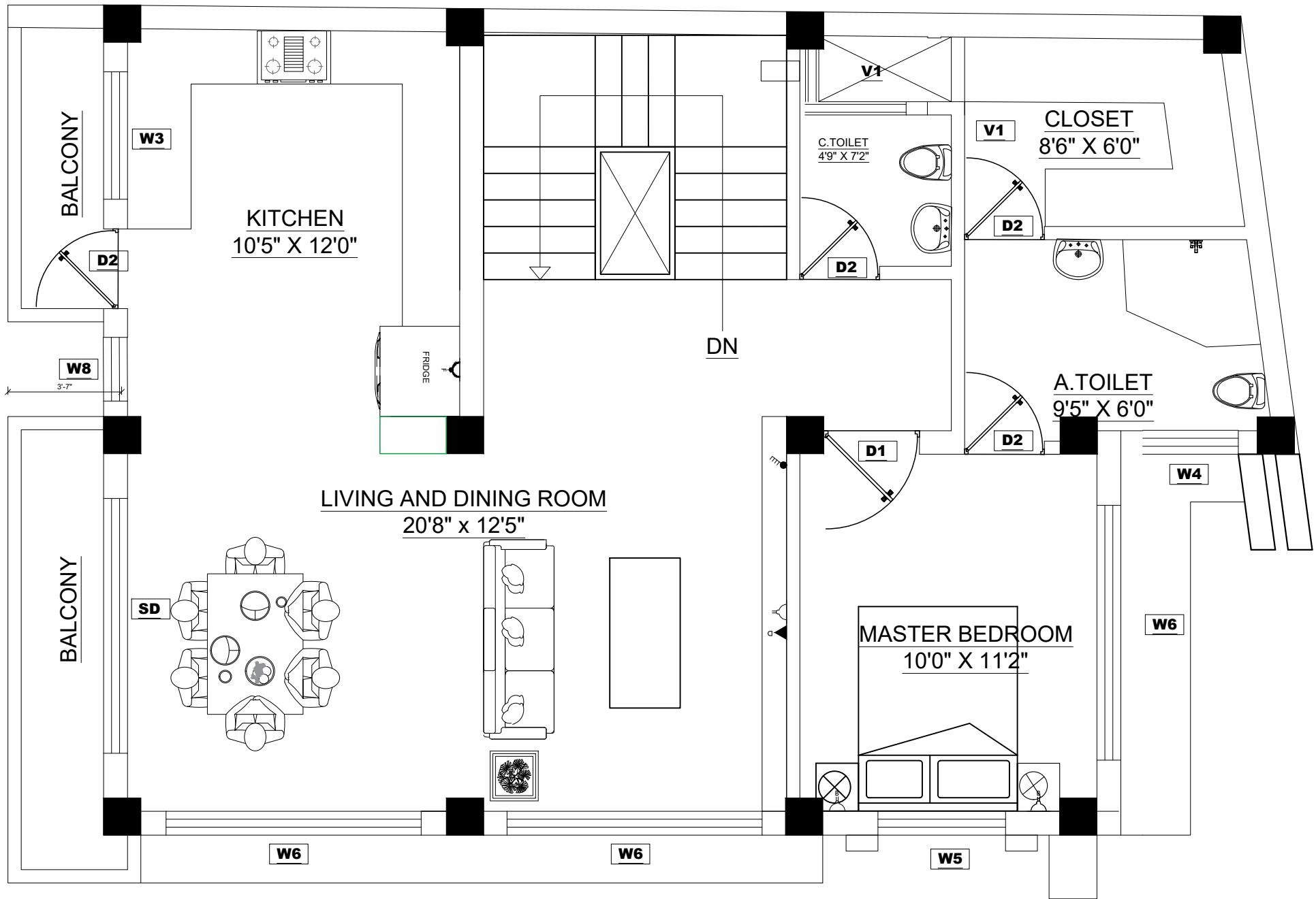
FIRST FLOOR PLAN AREA:897.83 SQ.FT
