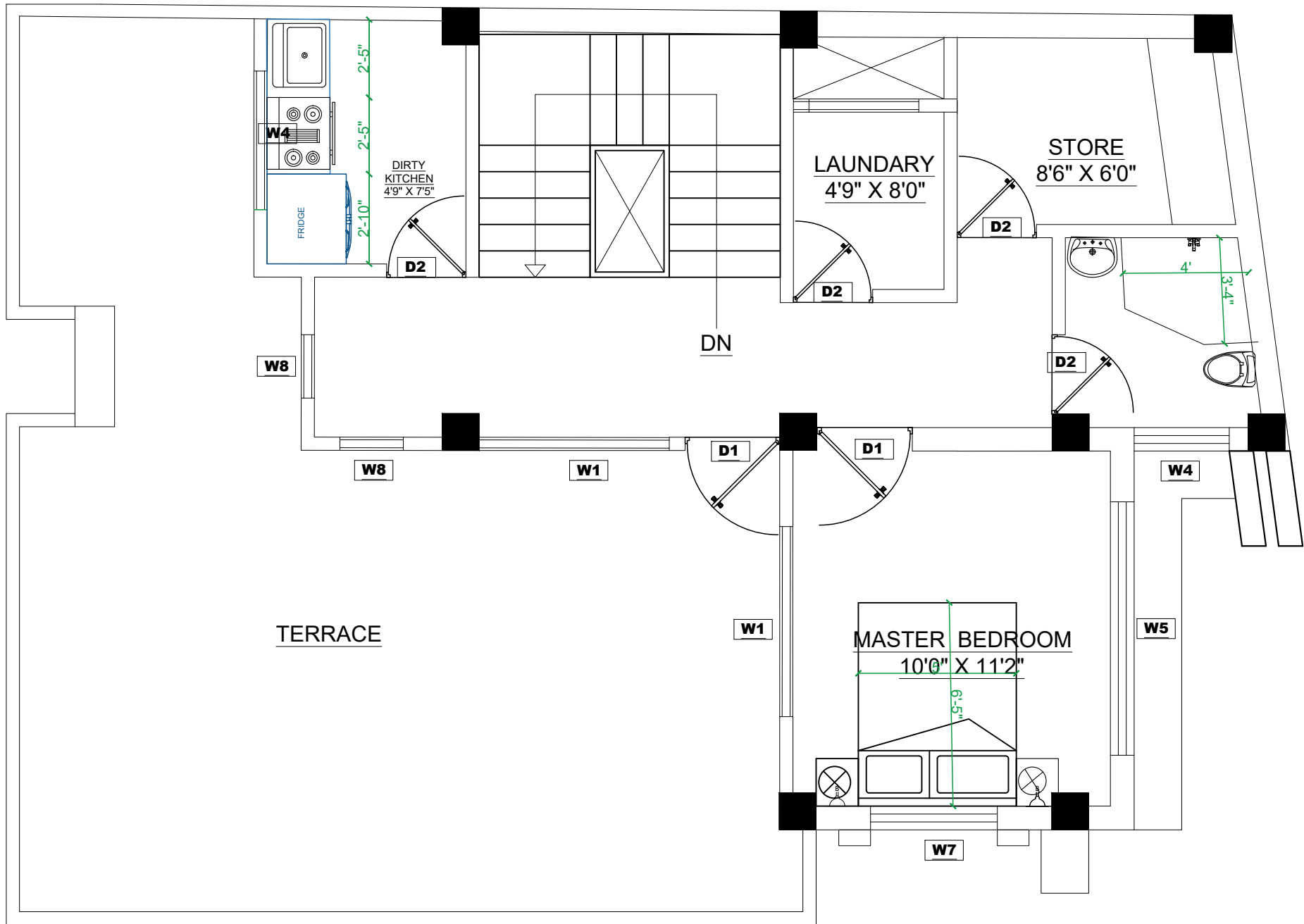
TOP FLOOR PLAN AREA:554.43 SQ.FT
